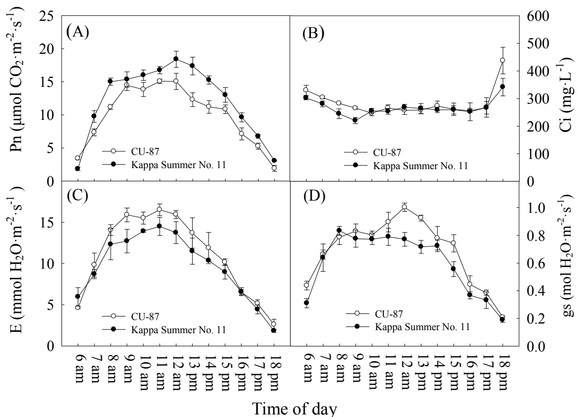
圖四、夏作花胡瓜淨光合作用(A)、細胞間隙 \text{CO}_2 濃度(B)、蒸散速率(C)及氣孔導度(D)之日變化 Fig. 4. Daily changes of cucumber net photosynthetic rate, Pn (A), cellular \text{CO}_2 concentration, Ci (B), transpiration rate, E (C), and stomatal conductance, gs (D) in summer. Date recorded: 2016.06.02
