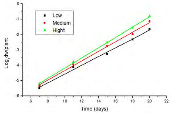
Figure 2. Dry matter accumulation of lettuce at 500 ppm \text{CO}_2 and 3 light intensities. (118, 166, 261 \mu\text{mol.m}^2.\text{s}^{-1} )
