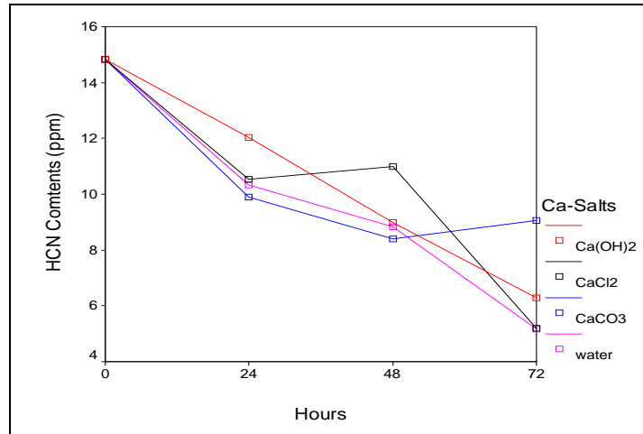
Figure 1. Effect of length of soaking on HCN content of jack bean.
