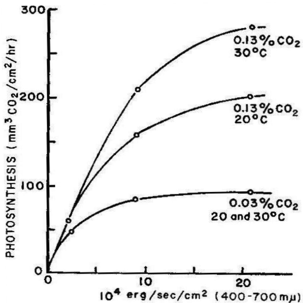
Figure 3. Effect of light intensity, temperature and \text{CO}_2 level on photosynthesis (after Gaastra 1959)
