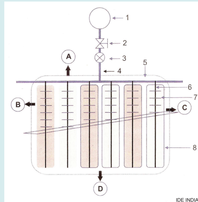
Figure 1. Layout of a typical drip irrigation system
