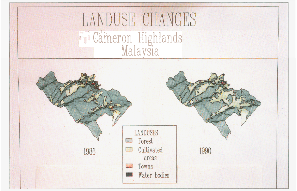
Plate 4. Landuse changes from 1986 to 1990 superimposed on a digital elevation model of the Cameron Highlands
